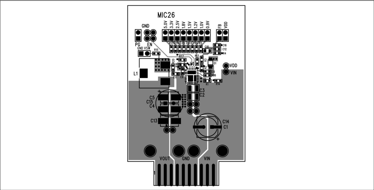
FIGURE 8-1: Evaluation Board Top Layer.
