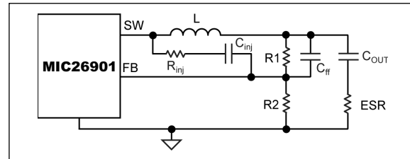
FIGURE 5-3: Invisible Ripple at FB.
