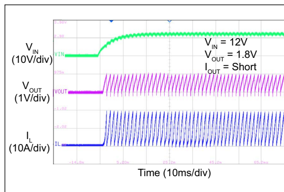
FIGURE 2-47: Power-Up into Short Circuit.
