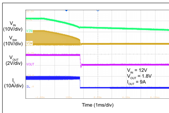
FIGURE 2-40: V_{IN} Turn-Off.
