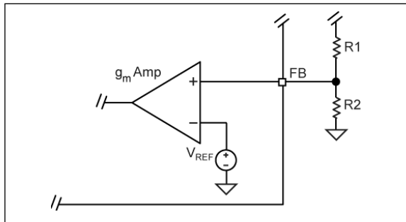
FIGURE 5-4: Voltage Divider Configuration.
