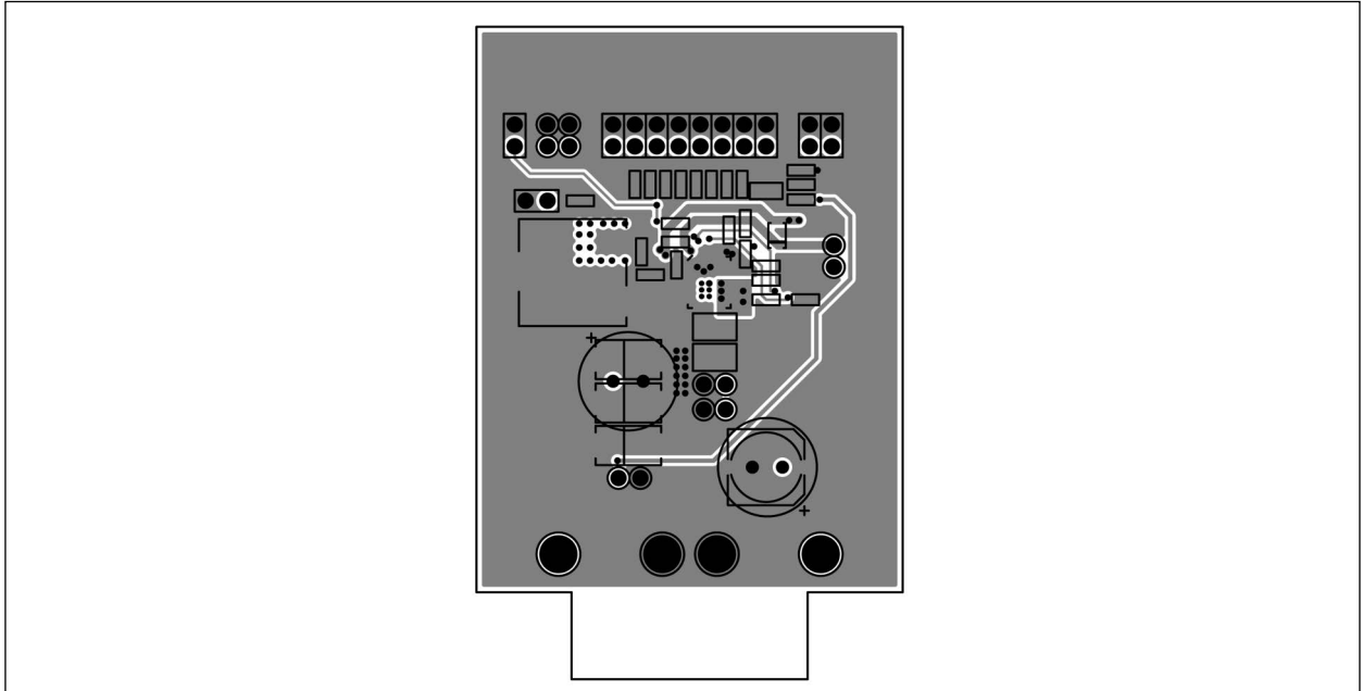
FIGURE 8-3: Evaluation Board Mid-Layer 2.
