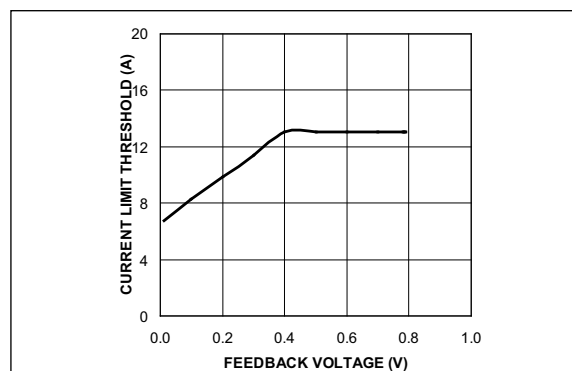
FIGURE 4-3: Current-Limit Foldback Characteristics.
