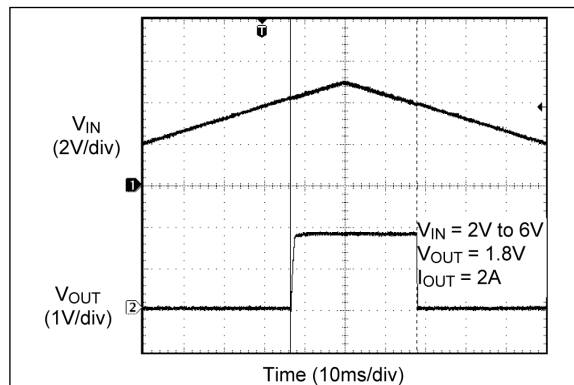
FIGURE 2-46: V IN UVLO Thresholds.
