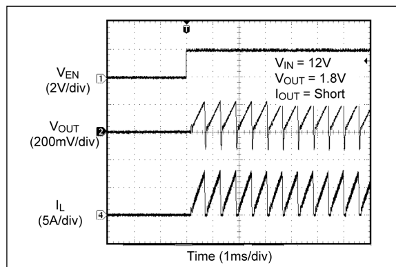
FIGURE 2-48: Enabled into Short.
