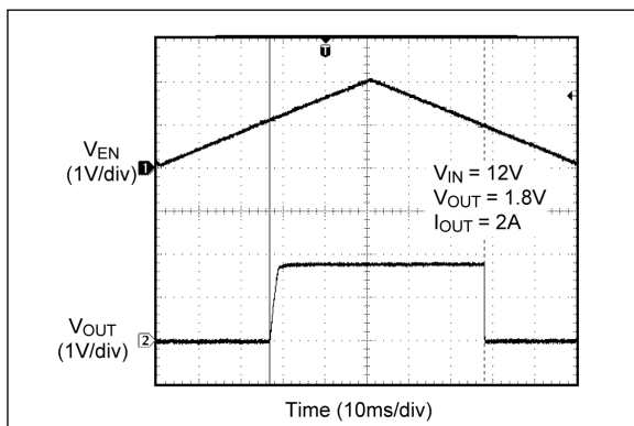
FIGURE 2-45: Enable Thresholds.
