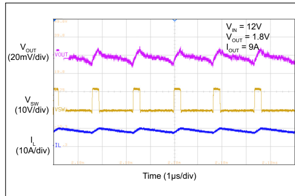
FIGURE 2-53: Switching Waveforms ( I_{OUT} = 9A ).
