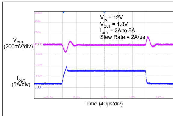
FIGURE 2-55: Transient Response (Slew Rate = 2A/ \mu s ).
