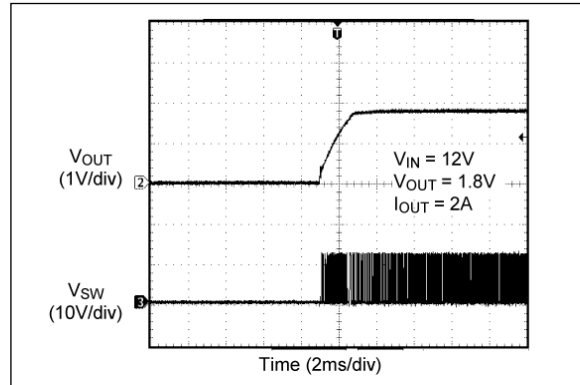
FIGURE 2-52: Output Recovery Time from Thermal Shutdown.
