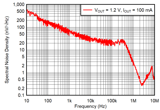
Figure 7-6. Noise Spectral Density
