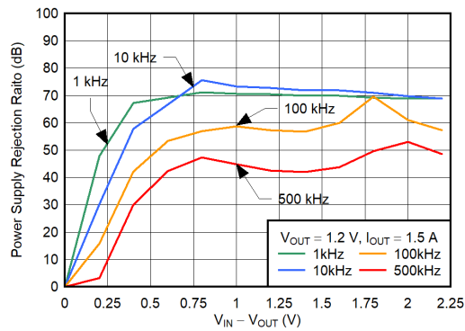
Figure 7-5. V_{IN} PSRR vs (V_{IN} - V_{OUT})
