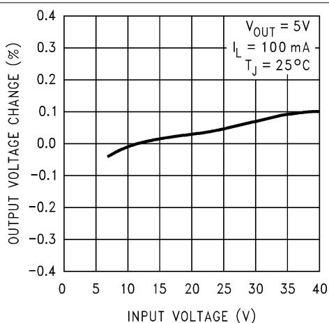
Figure 5-2. Line Regulation
