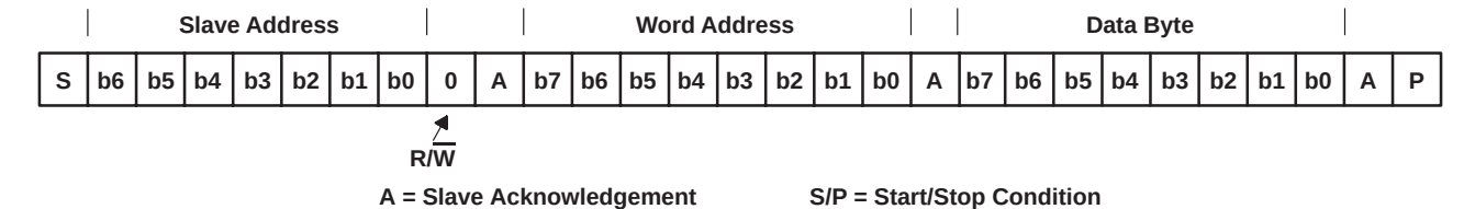
Figure 3-11. Serial-Bus Protocol – Byte Write
