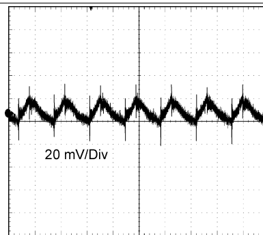
Figure 34. Output Ripple
