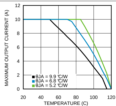
Figure 51. Thermal Derating
