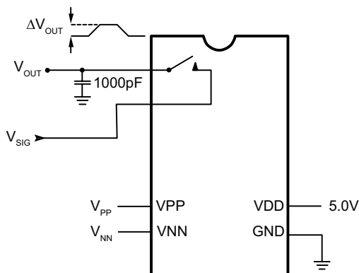
Q = 1000pF \cdot \Delta V_{OUT} Charge Injection
