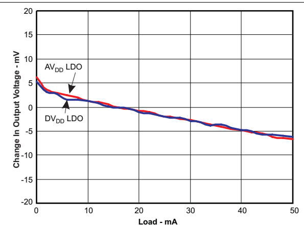
Figure 13. LDO Load Response
