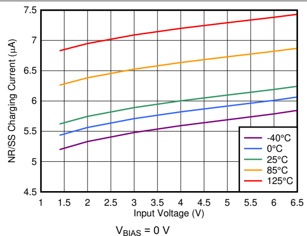
Figure 6-36. I_{NR/SS} Current vs Input Voltage
