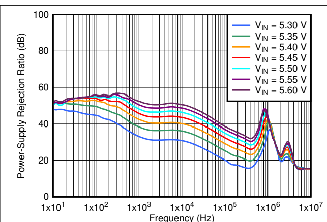
Figure 8-25. PSRR vs Frequency and V IN for V OUT = 5.0 V at I OUT = 3.0 A
