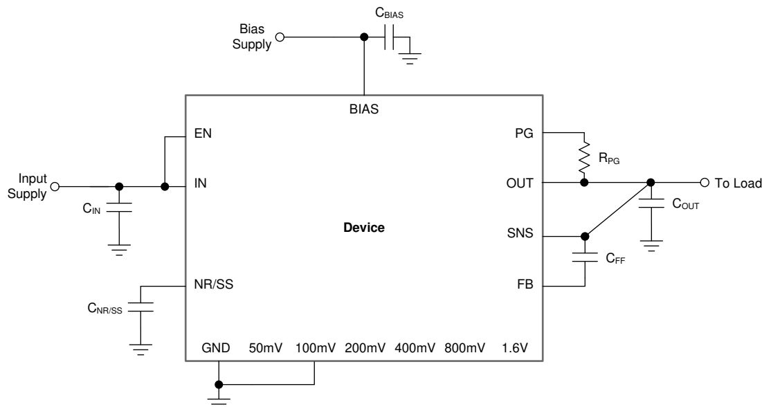
Figure 8-20. Typical Application
