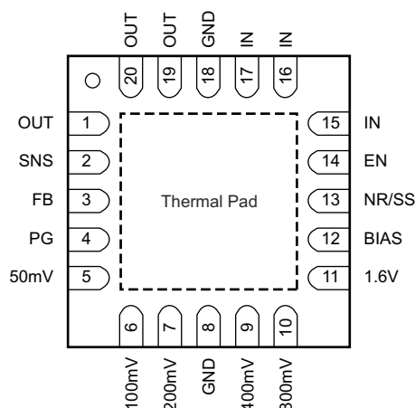
Figure 5-1. RGR Package, 3.5-mm × 3.5-mm, 20-Pin VQFN, Top View
