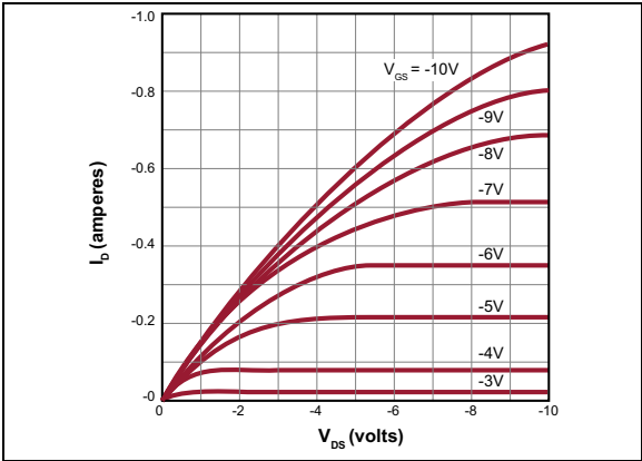
FIGURE 2-4: Saturation Characteristics.
