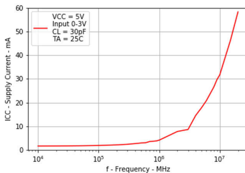
Figure 5-14. Supply Current vs Frequency
