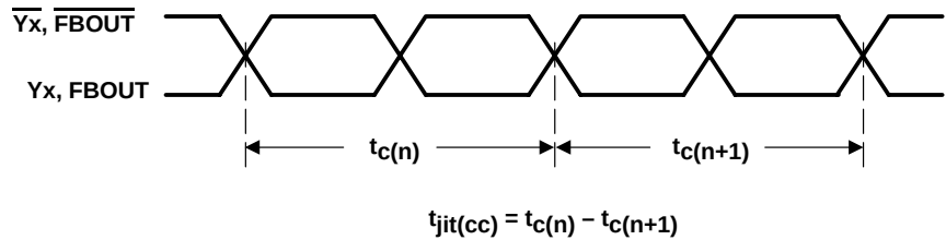
Figure 2. Cycle-to-Cycle Jitter
