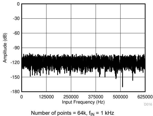
Figure 6-33. Typical FFT Plot (All Ranges) for the ADS8661
