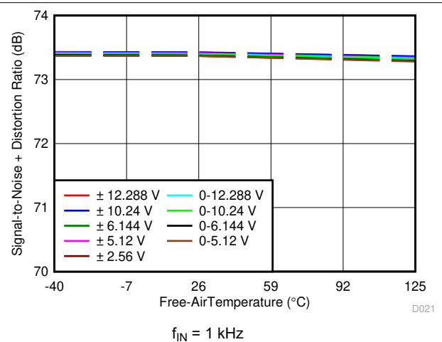
Figure 6-38. SINAD vs Temperature
