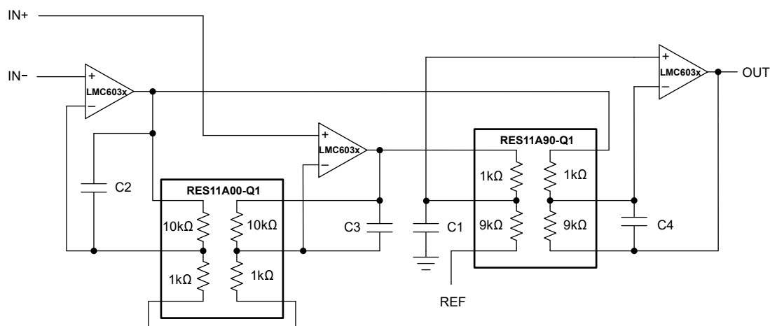
Figure 6-7. Improved Instrumentation Amplifier With RES11A
