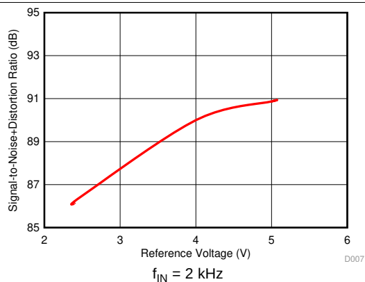
Figure 8. SINAD vs Reference Voltage
