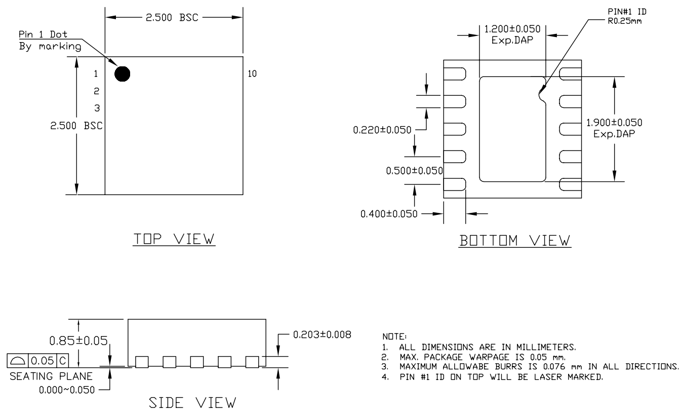
10-Pin Package MLF® (ML)
