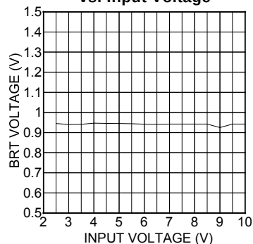
BRT Voltage vs. Input Voltage
