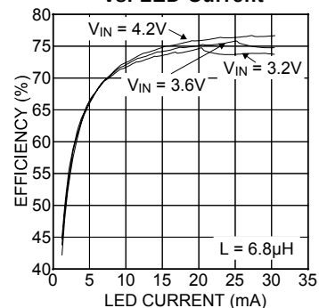
Efficiency for 10 LEDs vs. LED Current
