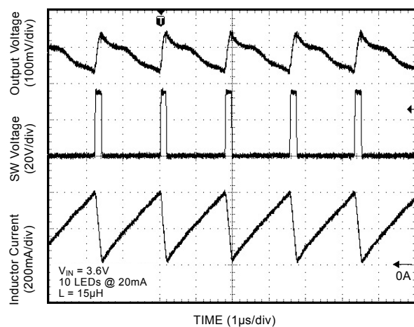
Waveform 2
