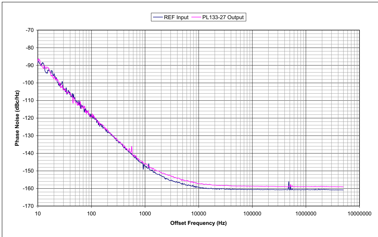
FIGURE 2-1: PL133-27 Additive Phase Jitter. V_{DD} = 3.3V , CLK = 26 MHz, Integration Range: 12 kHz to 5 MHz, 0.127 ps Typical.
