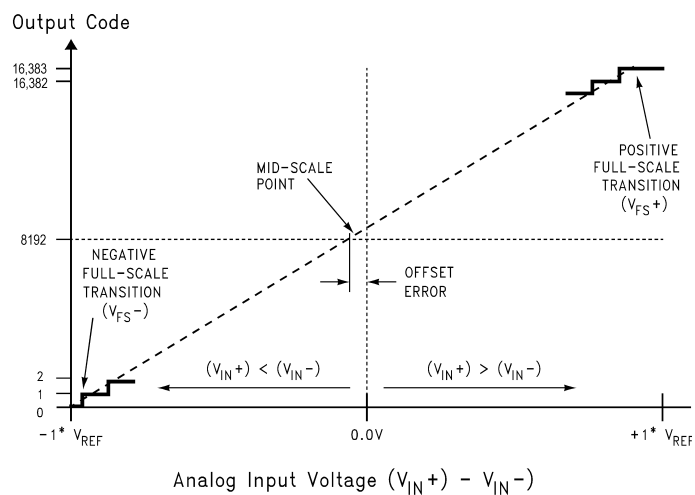
Figure 2. Transfer Characteristic
