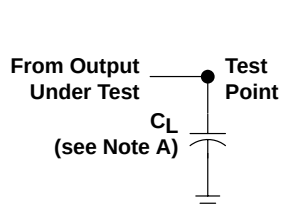
LOAD CIRCUIT FOR TOTEM-POLE OUTPUTS
