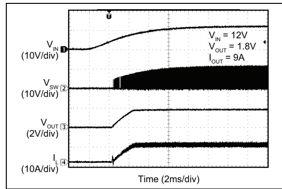
FIGURE 2-35: V_{IN} Soft Turn-On.
