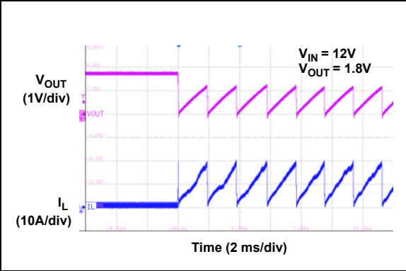
FIGURE 2-45: Short Circuit.
