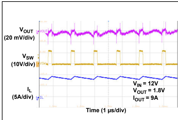
FIGURE 2-49: Switching Waveforms, I_{OUT} = 9A .
