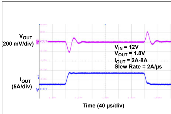
FIGURE 2-51: Transient Response.
