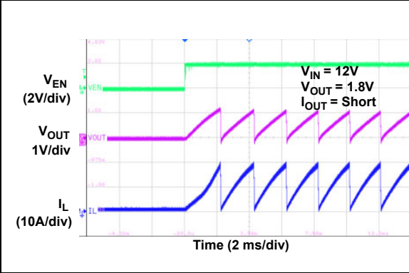
FIGURE 2-44: Enabled into Short.
