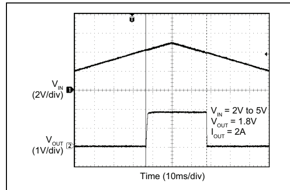
FIGURE 2-42: V_{IN} UVLO Thresholds.
