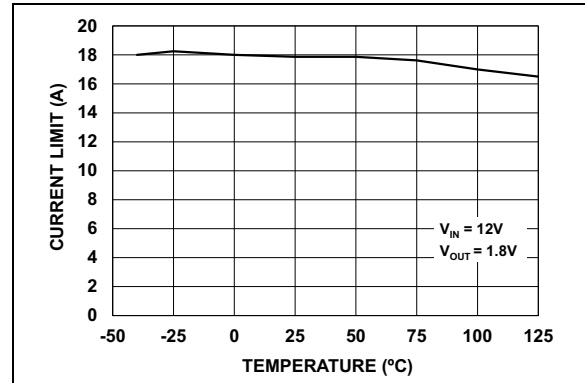
FIGURE 2-18: Output Current Limit vs. Temperature.
