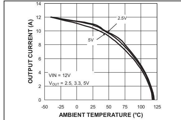
FIGURE 2-34: Thermal Derating vs. Ambient Temperature (Note 1).
