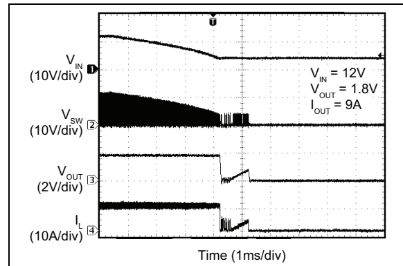
FIGURE 2-36: V_{IN} Soft Turn-Off.
