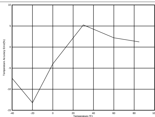
Figure 8. Temperature Accuracy
