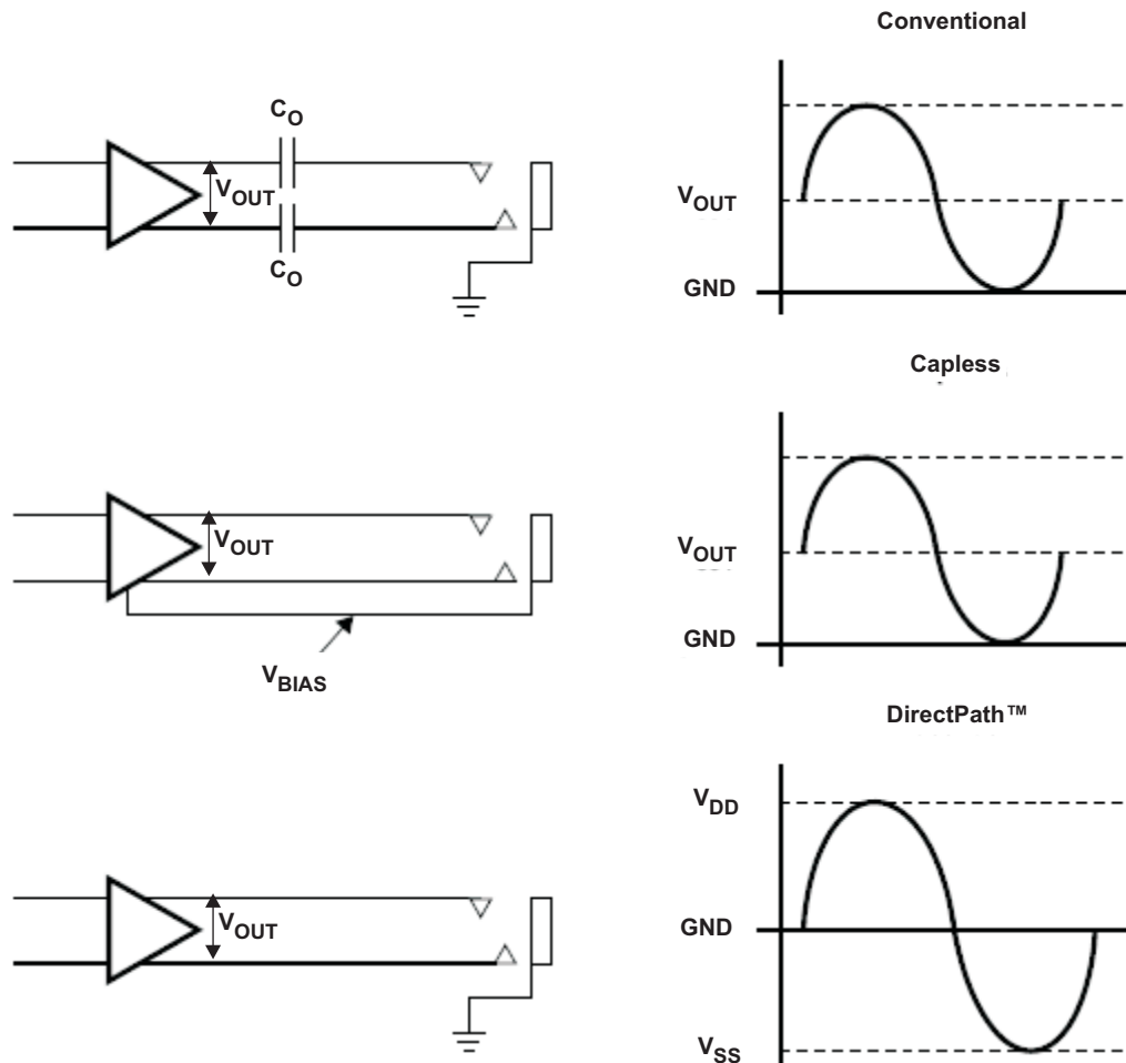
Figure 31. Amplifier Applications
