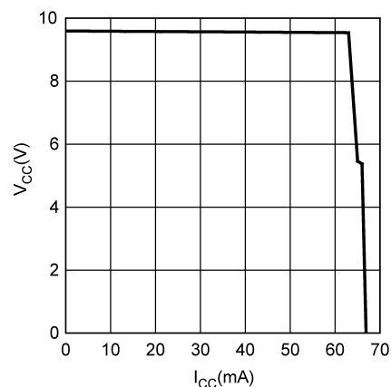
Figure 5-2. V_{CC} vs I_{CC}
