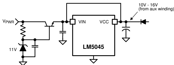
Figure 7-3. Start-Up Regulator For V_{PWR} > 100 V
