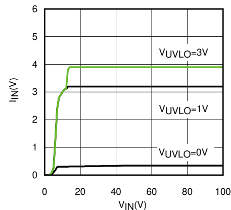
Figure 5-4. I_{IN} vs V_{IN}
