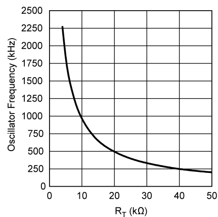
Figure 5-6. Oscillator Frequency vs R_T
