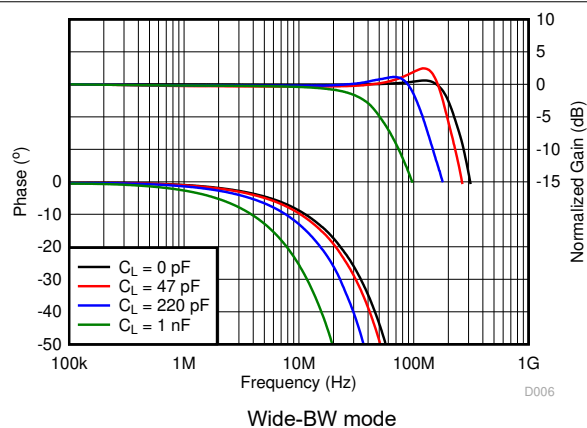
Figure 6-24. Gain and Phase vs Frequency and Load Capacitance Wide-BW mode
