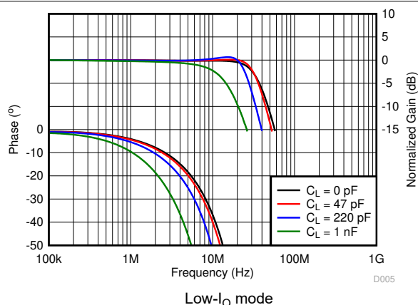
Figure 6-23. Gain and Phase vs Frequency and Load Capacitance Low- I_Q mode
