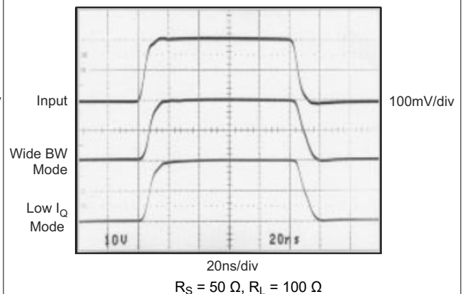
Figure 6-18. Large-Signal Response
