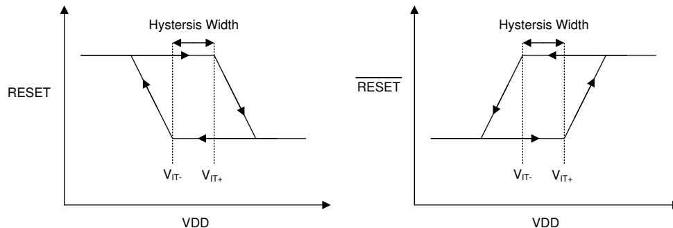
Figure 7-1. Hysteresis Diagram
