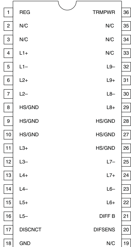
QSOP-36 (TOP VIEW) MWP Package
