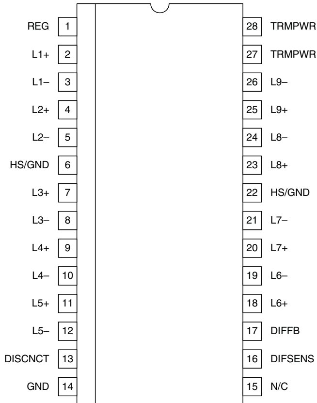
TSSOP-28 (TOP VIEW) PWP Package
