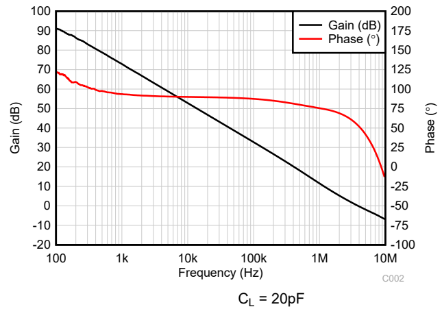
Figure 5-16. Open-Loop Gain and Phase vs Frequency V_S = \pm 20V R_L = 10\Omega , New Die
