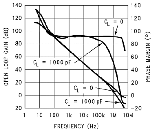
Figure 5-15. Gain and Phase, 2.7V Supply
