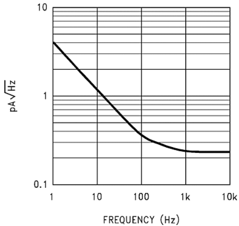
Figure 5-13. Current Noise vs Frequency
