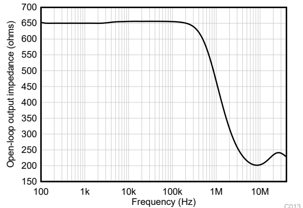
Figure 5-20. Open-Loop Output Impedance vs Frequency V_S = \pm 20V , New Die
