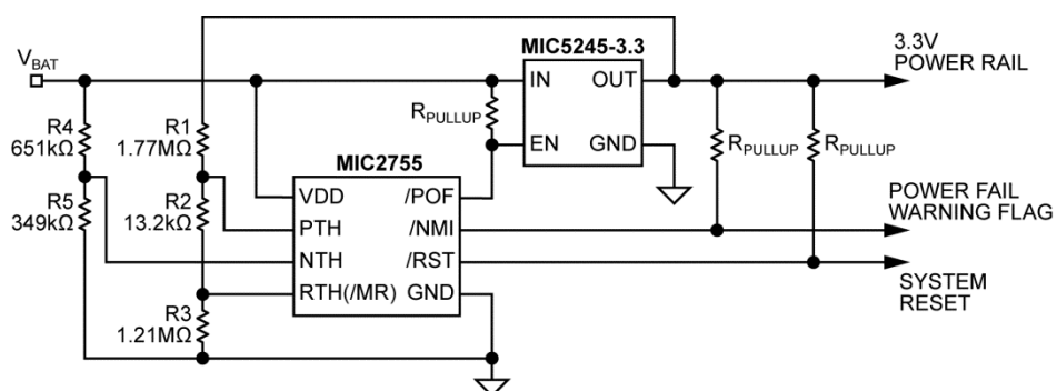
Figure 6. Voltage Supervisor with Power Fail Warning
