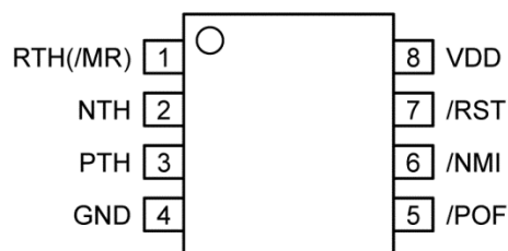
8-Pin MSOP (MM) (Top View)
