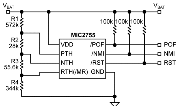
Figure 1. Example Circuit without Manual Reset
