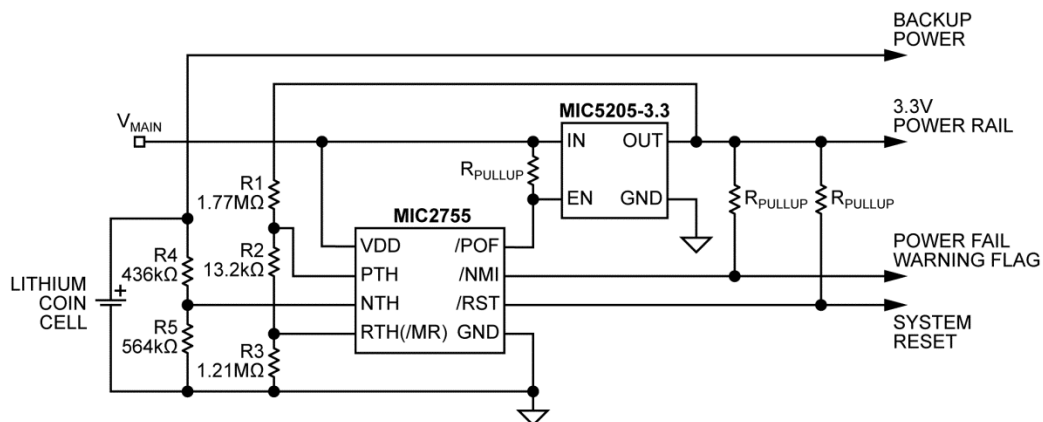
Figure 5. Voltage Supervisor and Backup Battery Monitor
