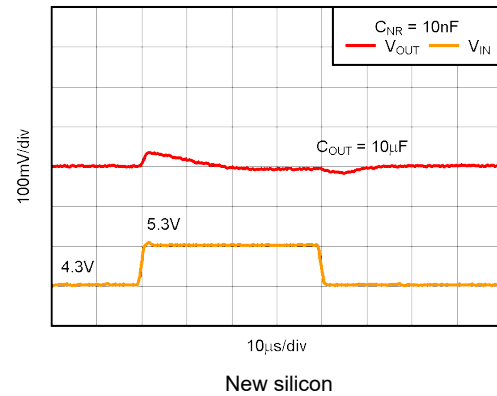
Figure 5-38. TPS73733 Line Transient Response
