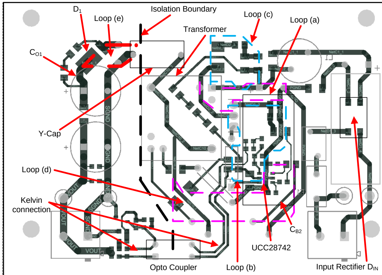
Figure 26. Layout Example
