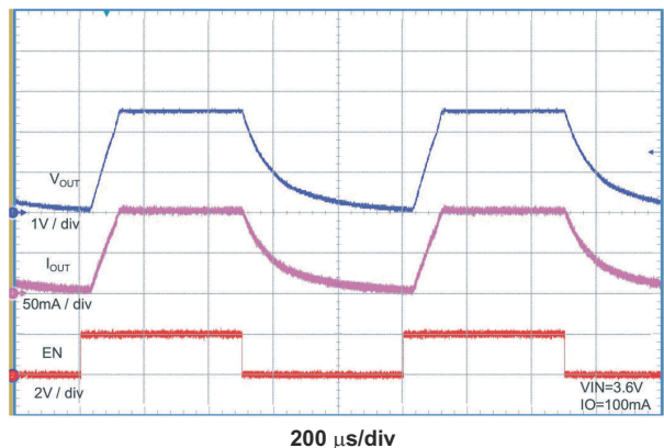
Figure 7-15. Enable / Disable V_{IN} = 3.6V , I_O = 100mA
