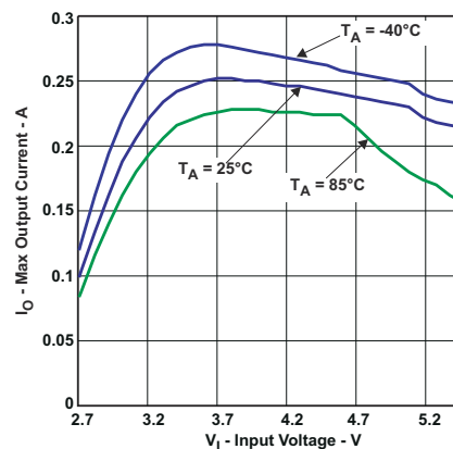
Figure 5-2. Maximum Output Current vs Input Voltage at Temperature
