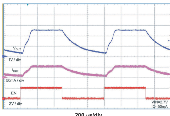
Figure 7-14. Enable / Disable V_{IN} = 2.7V , I_O = 50mA
