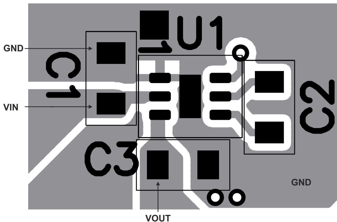
Figure 7-18. Recommended PCB Layout
