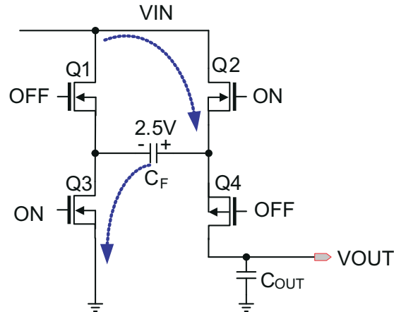
Figure 6-1. Charging Mode
