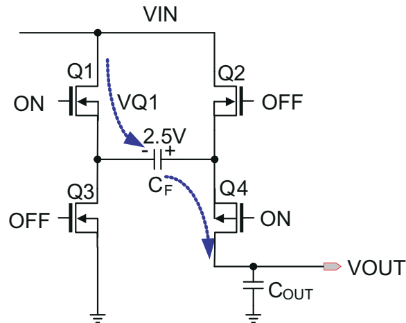
Figure 6-2. Discharging Mode
