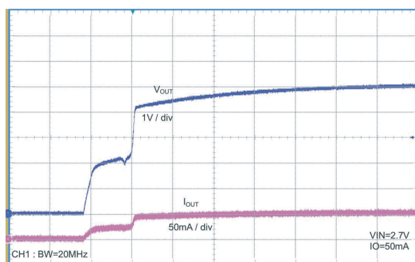
Figure 7-12. Power On V_{IN} = 2.7V , I_O = 50mA
