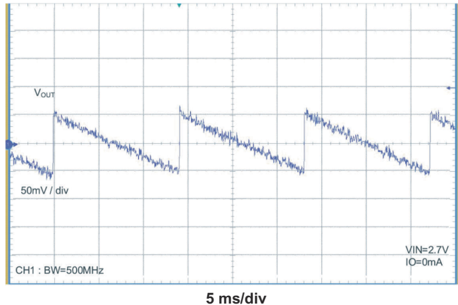
Figure 7-8. Output Ripple Voltage (Skip Mode) V_{IN} = 2.7V , I_O = 0mA
