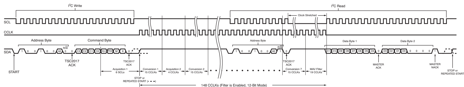
Figure 33. Data Acquisition Cycle (Filter Enabled)
