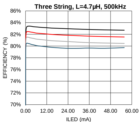
Figure 50. Efficiency vs I_{LED}
