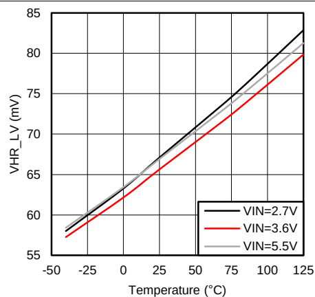
Figure 9. V_{HR\_LV} vs Temperature
