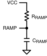
Figure 6-6. R_{RAMP} to V_{CC} for V_{OUT} > 7.5\text{ V}
