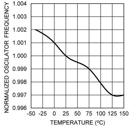
Figure 5-2. Oscillator Frequency vs Temperature (Q0) F_{Osc} = 200 \text{ kHz}
