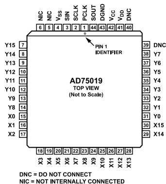
Figure 3. Pin Configuration
