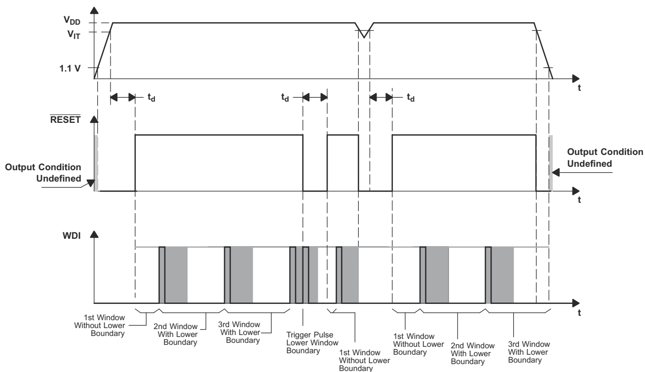
Figure 6-1. Timing Diagram
