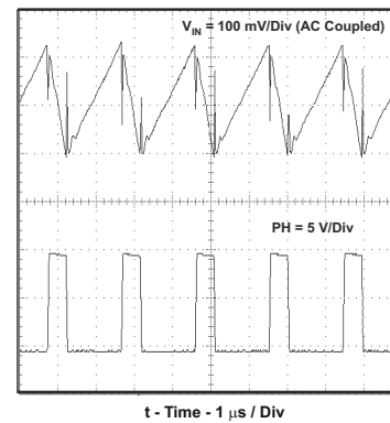
Figure 7-5. Input Voltage Ripple and PH Node, I_O = 3\text{A}
