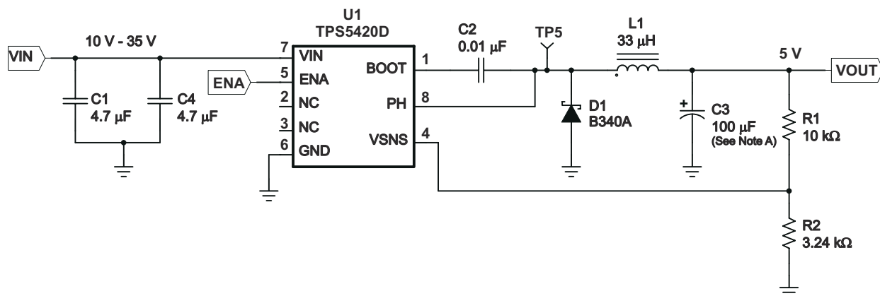
Figure 7-1. Application Circuit, 10V — 35V to 5V
