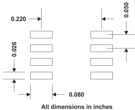
Figure 7-13. TPS5420 Land Pattern
