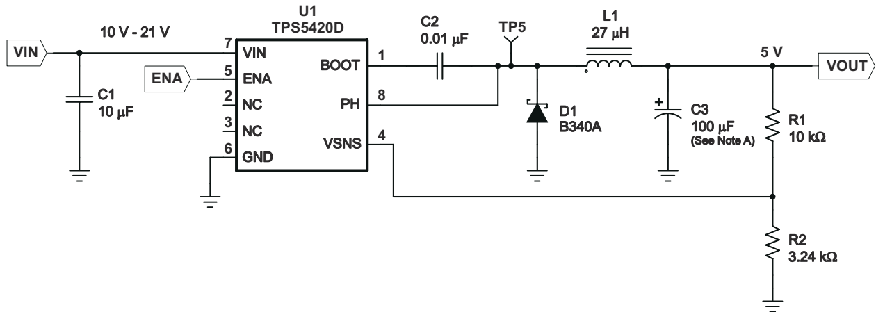
Figure 7-10. 10V — 21V Input to 5V Output Application Circuit
