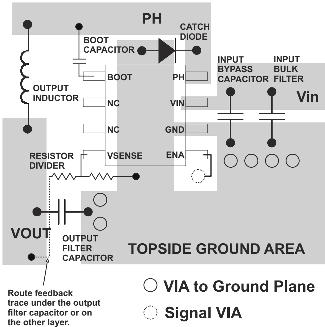
Figure 7-12. Design Layout
