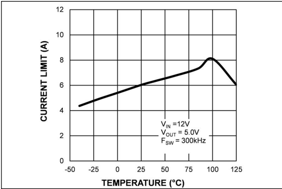
FIGURE 2-12: Output Peak Current Limit vs. Temperature (MIC28513-1).
