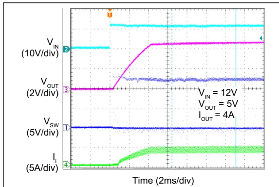
FIGURE 2-26: V_{IN} Turn-On.
