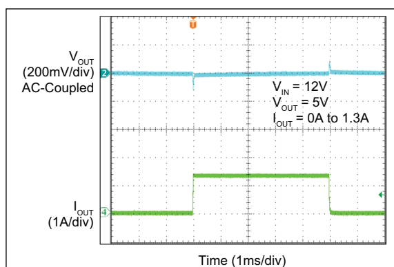
FIGURE 2-48: MIC28513-2 Load Transient Response (0A to 1.3A).
