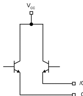
Figure 4. Simplified LVPECL Output Stage
