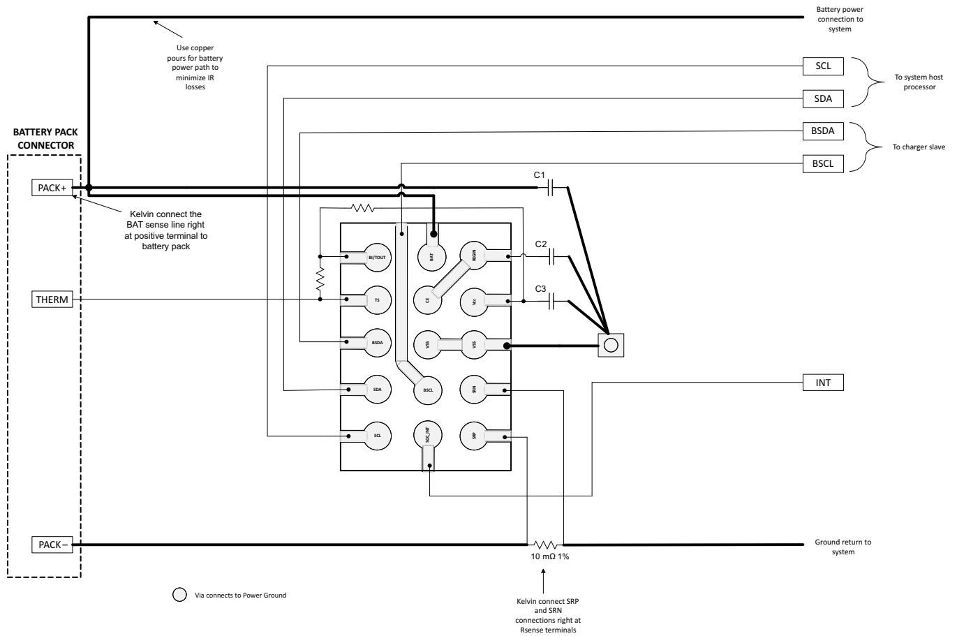
Figure 17. Layout Schematic
