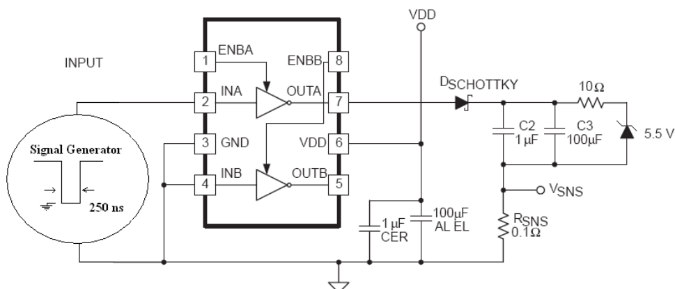
Figure 26. Current Sourcing
