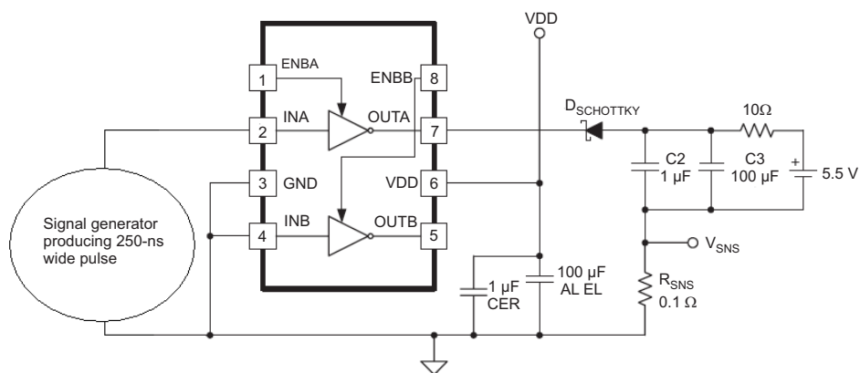
Figure 25. Current Sinking
