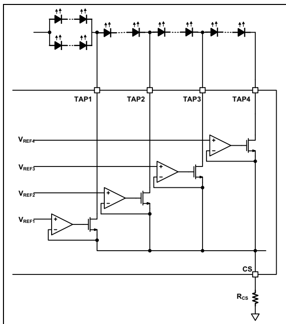
FIGURE 3-1: Tap Commutation.
