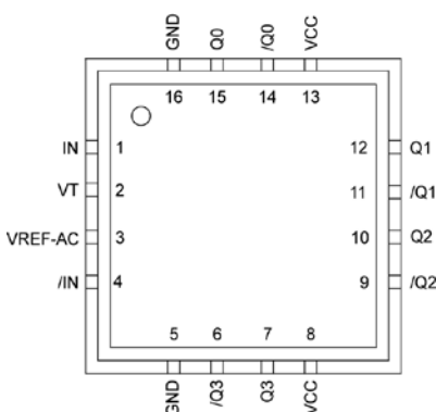
16-Pin QFN
