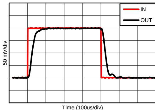
Figure 27. Pulse Response, 200mVpp at 1.8 V
