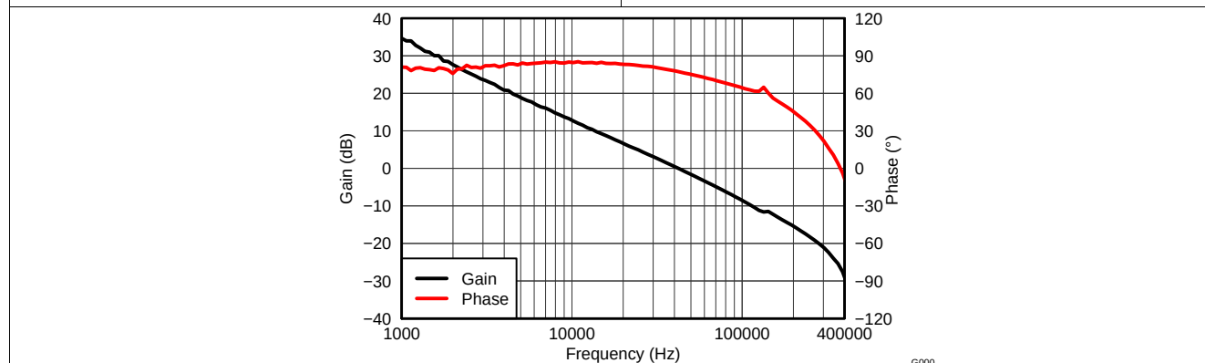
Figure 10. V OUT =1.8 V, I OUT =3 A, C OUT1 = 100 \mu F ceramic, C OUT2 = 100 \mu F ceramic, f SW = 480 kHz
